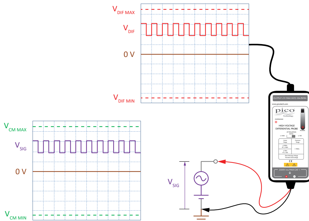
Figure 3 - Single-ended measurement
